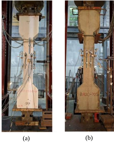
Fig. 4 Testing arrangements: (a) concentric and (b) eccentric test set up.
