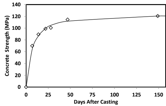
Fig. 3 Concrete compressive strength versus days after casting.
