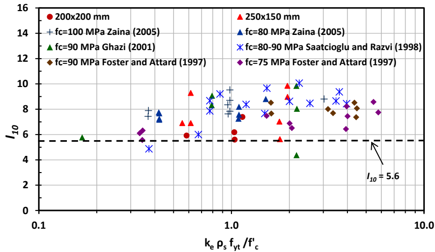
Fig. 7 Ductility index of I_{10} versus the confinement parameter k_e \rho_s f_{yt} / f'_c .
