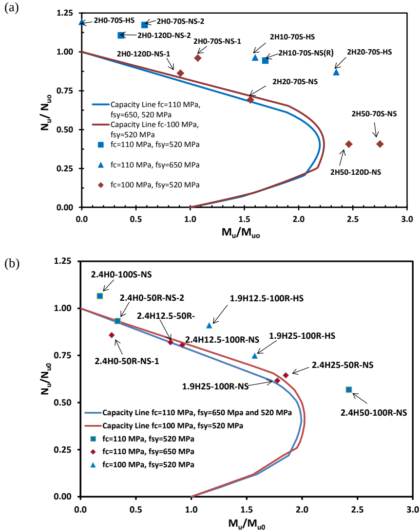
Fig. 6 Column capacities compared to AS3600-2018 interaction diagram: (a) 200 \times 200 mm section; (b) 250 \times 150 mm section (tested in this study and that of Parvez et al., 2017).
