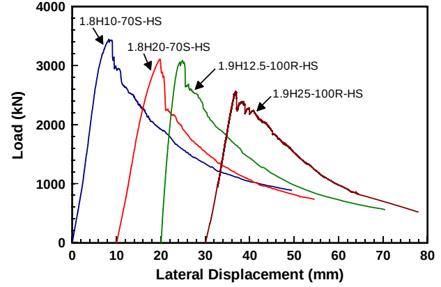
Fig. 5 Load versus lateral deflection for HSC-HSS columns tested in this study.
