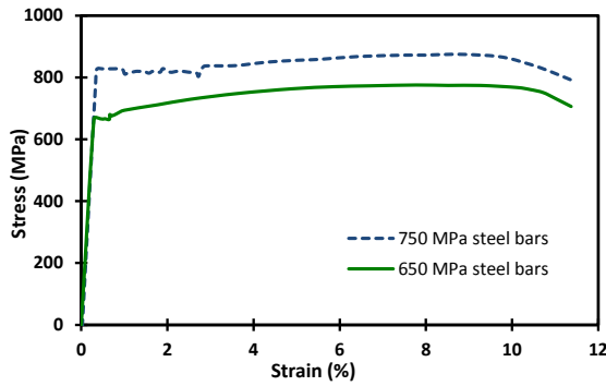
Fig. 2 Stress-strain curve for 670 and 810 MPa bars of 10.7 mm and 5.5 mm diameter, respectively.
