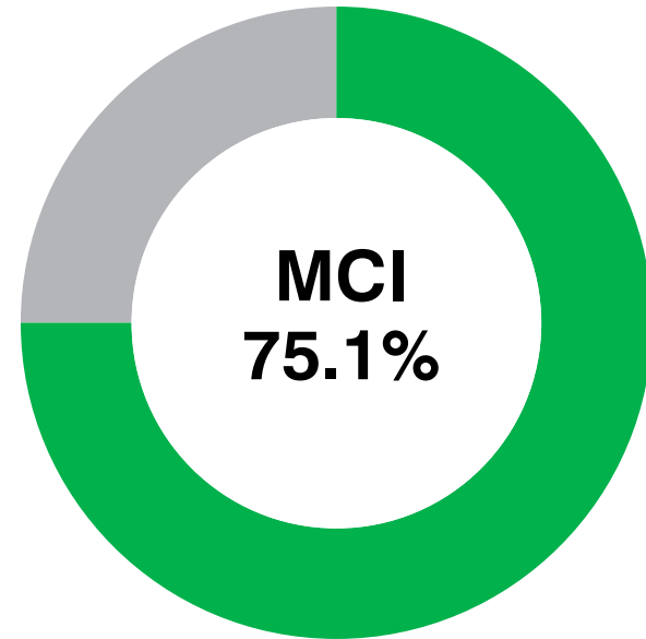
Figure 4. MCI score
