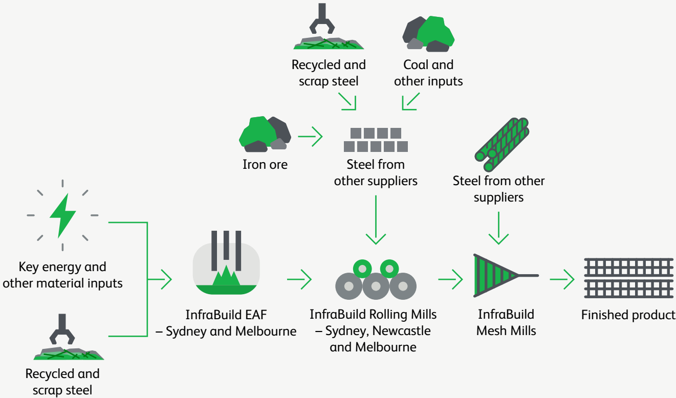
Figure 2. Basic manufacturing process
