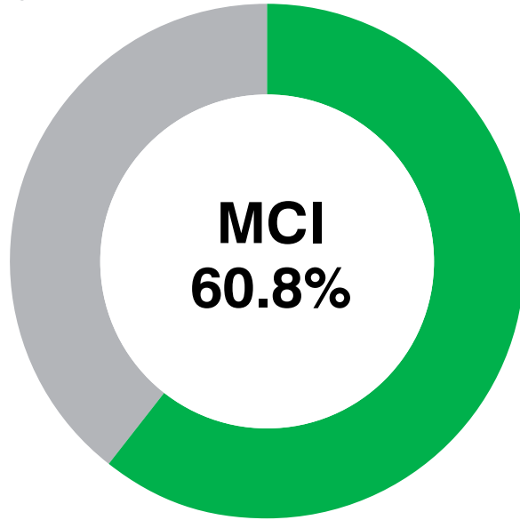
Figure 4. MCI score
