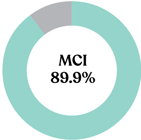
Figure 4. MCI score
