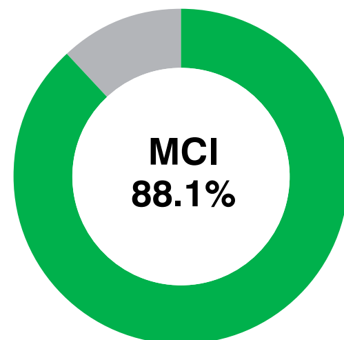
Figure 4. MCI score
