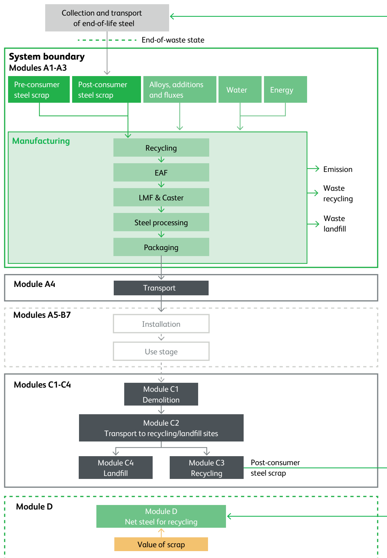
Figure 3. System boundary diagram
